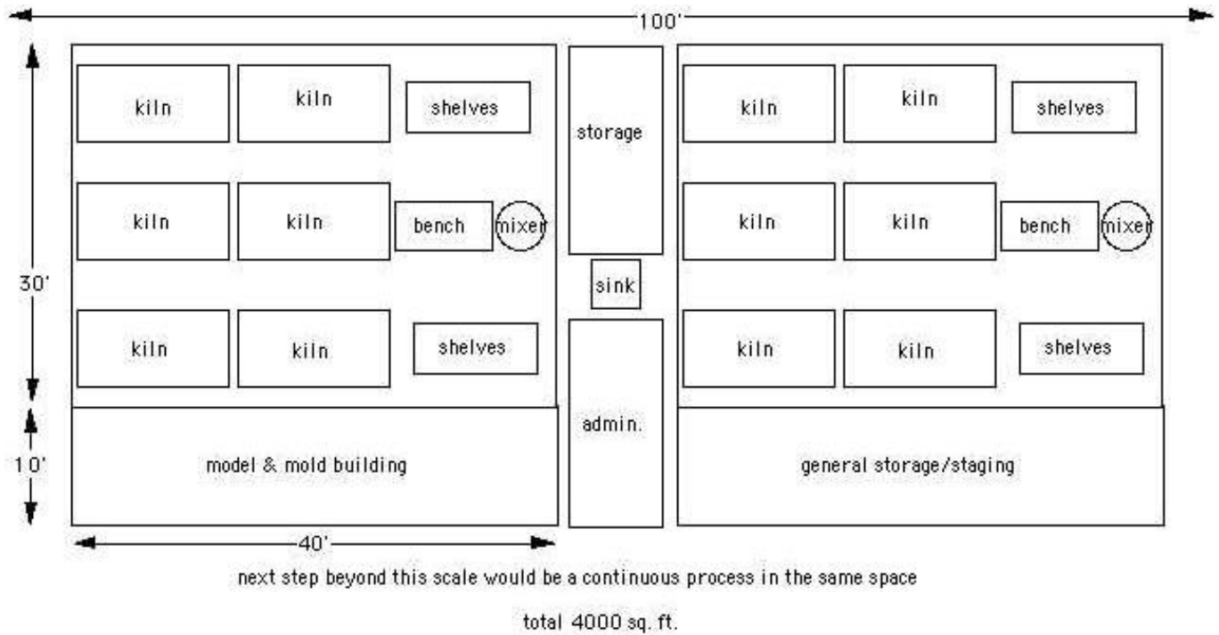
Figure 10 - Possible Kiln Set-Up
