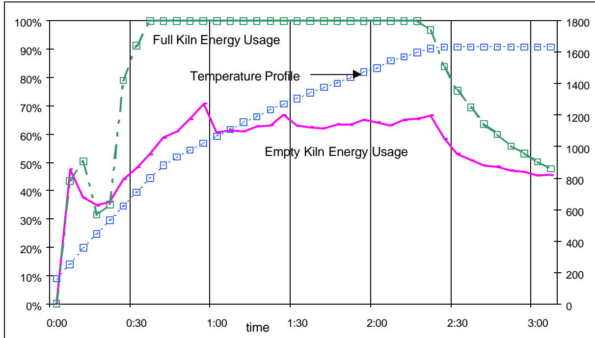
Figure 9 - Energy Use During Empty and Full Firing.
