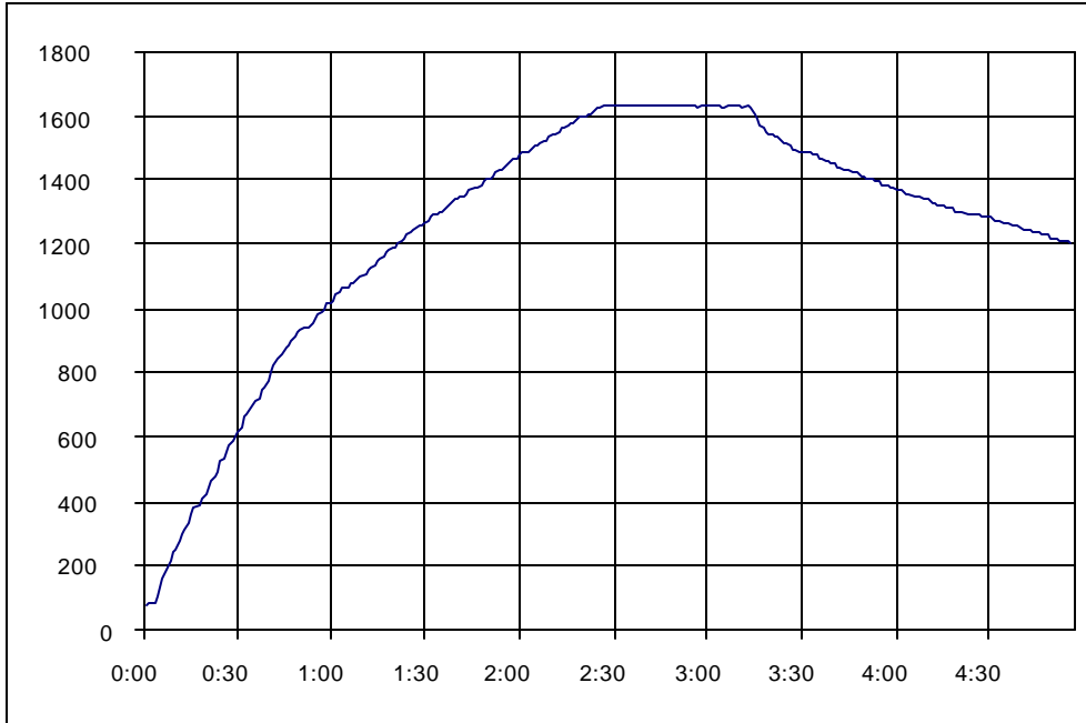
Figure 6 - Temperature Profile for Firings. (y-axis is temperature in F, x-axis is Time)
