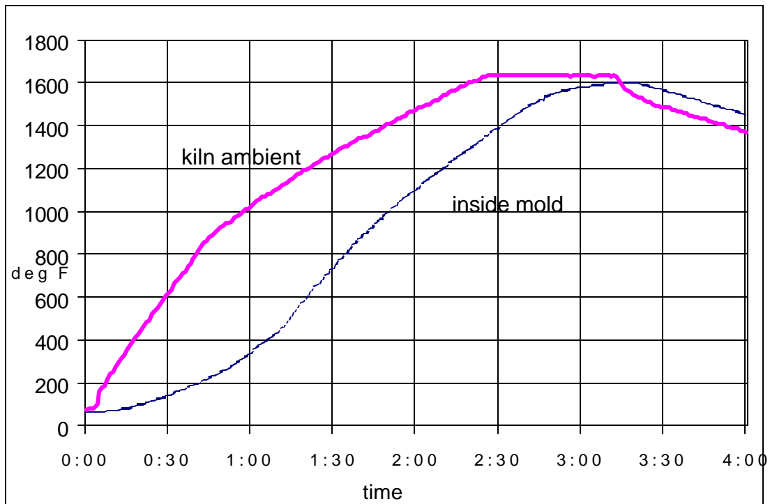
Figure 8 - Temperature Profile Inside Mold and Kiln Ambient
